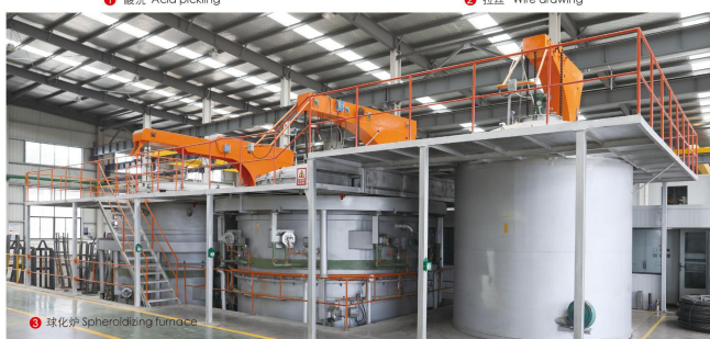
3 球化炉 Spheroidizing furnace
